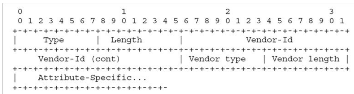
FIGURE 9 VSA fields
