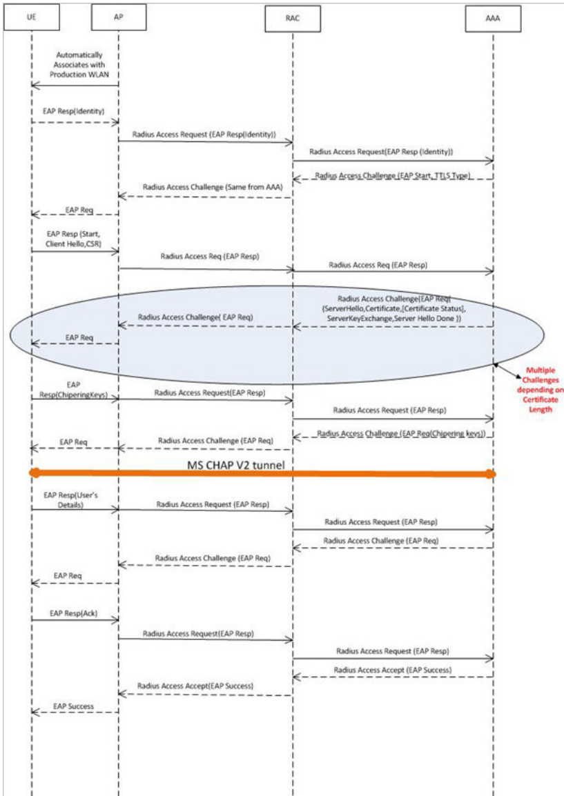
FIGURE 6 R2 device access authentication
