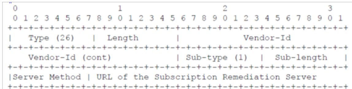
FIGURE 7 Hotspot 2.0 VSA fields
